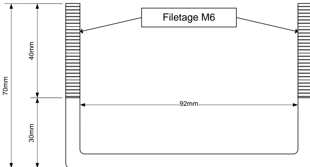
Inox \varnothing 6 mm – Filetage M6 – 4x
