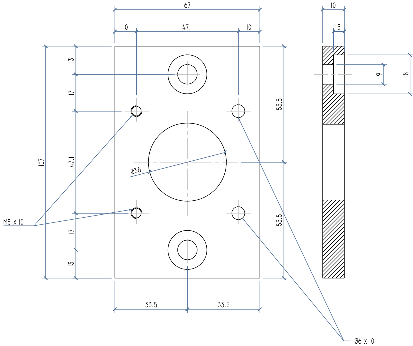
PLAQUE ALUMINIUM
