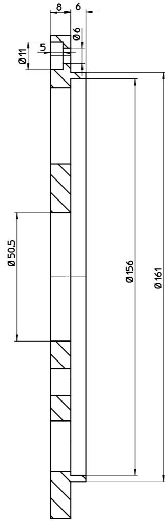
Cross-section A-A
